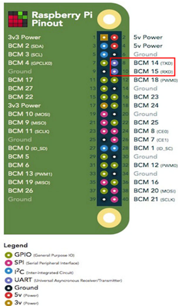
Figure 1: Pin-outs
