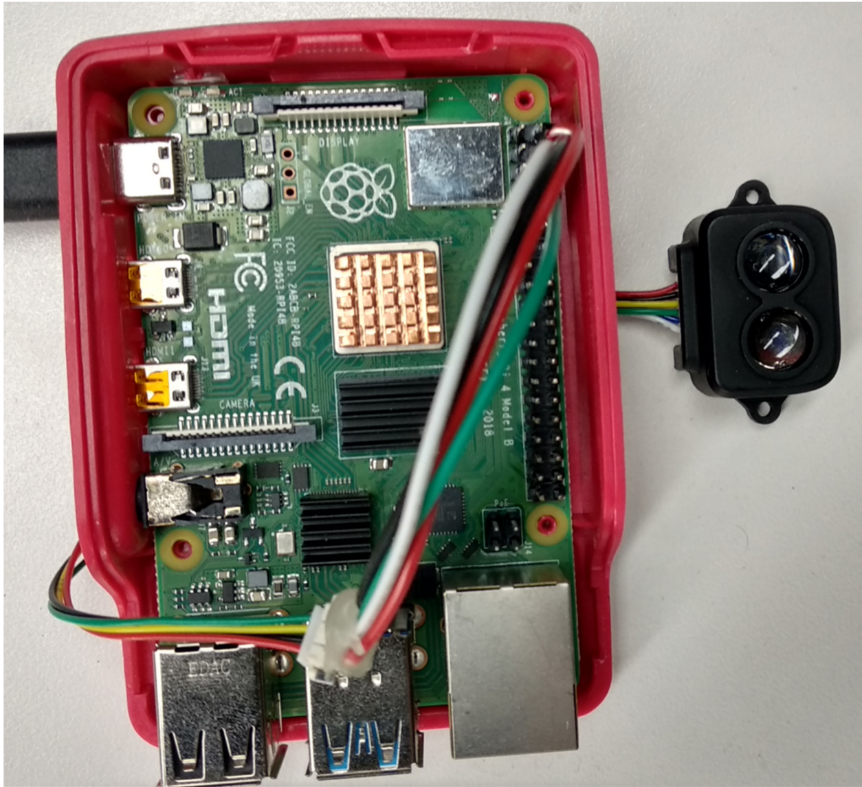
Figure 5: Actual connection
