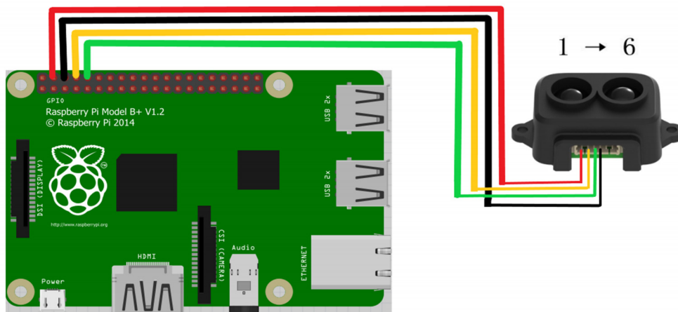
Figure 4: Schematic
